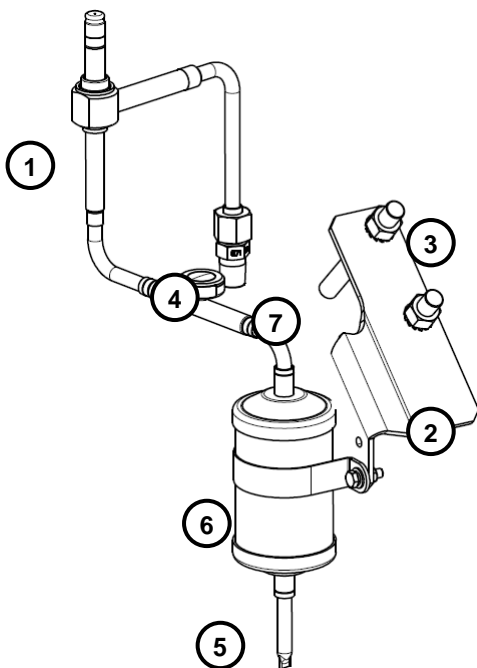
Figure 4: Injection valve kits when assembled
