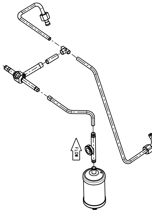
Figure 3: Injection valve kit for 6M* compressors
