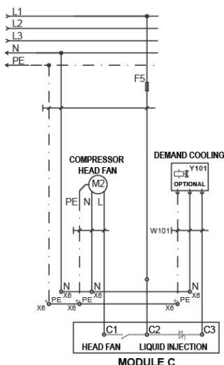
Figure 7: Wiring diagram for liquid injection and/or head fan monitored via module C
