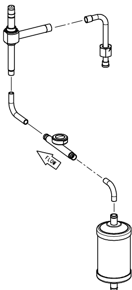
Figure 2: Injection valve kit parts for 4M* compressors
