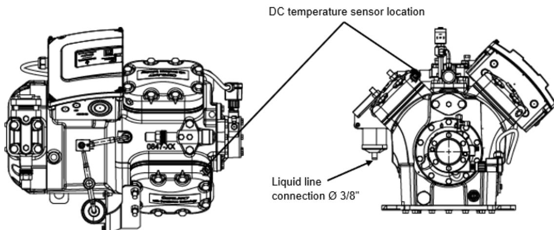
Figure 8: Injection parts on 4M* compressors
