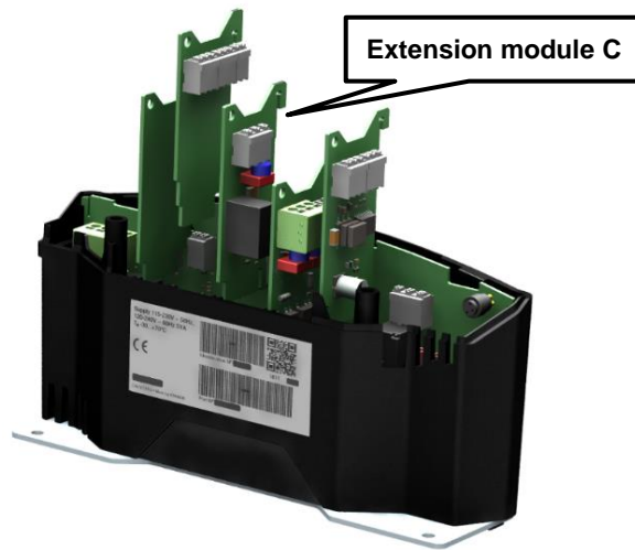
Figure 6: Copeland Compressor Electronic with modules
