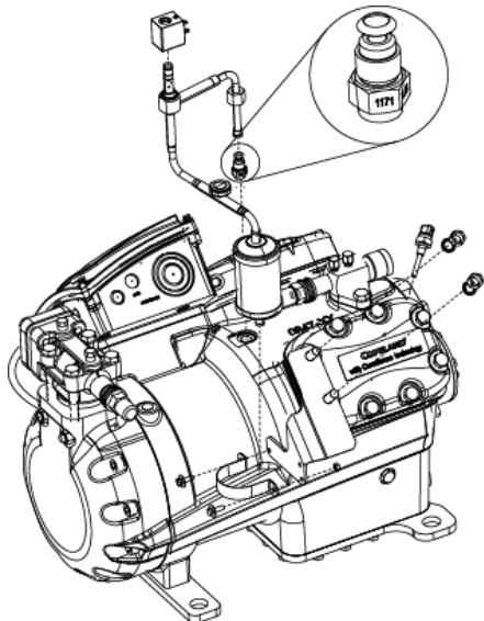
Figure 8: Injection parts on 4M* compressors
