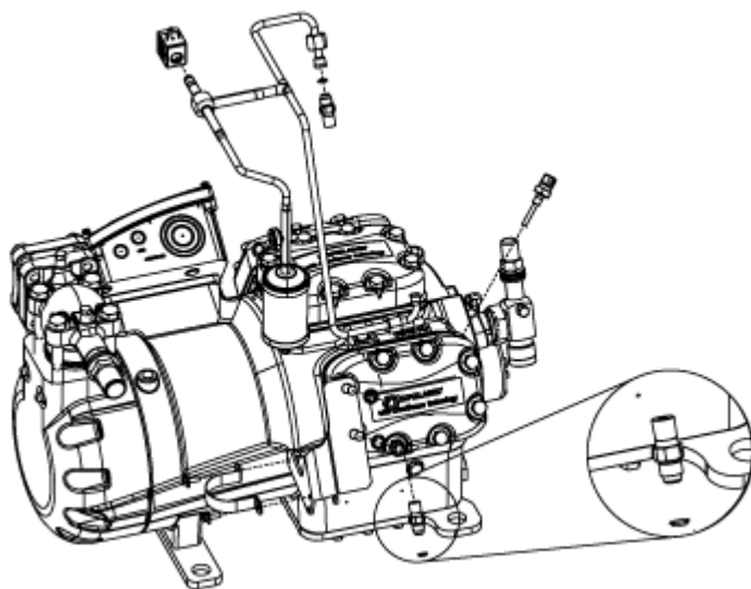
Figure 9: Injection parts on 6M* compressors
