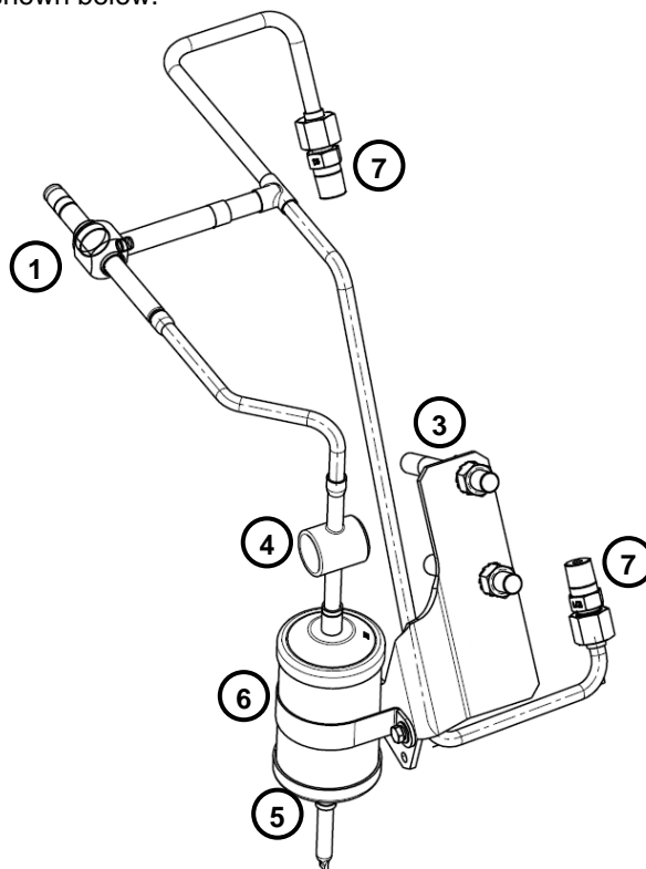
Figure 3: Injection valve kit for 6M* compressors
